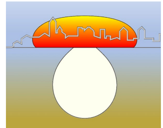
Profiles of sessile (up, Bo=5 ) and pendant (down, Bo=0.2 ) drops deformed by gravity on a hydrophobic substrate (not to scale).
