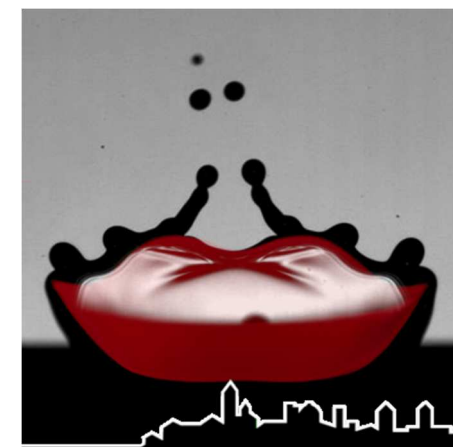
Crown formed after inclined drop impact on liquid film.
